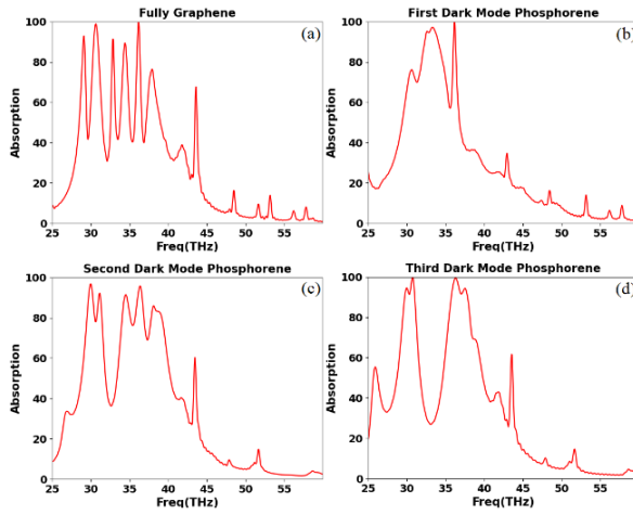
Figure 7. Absorption profiles of the structure
