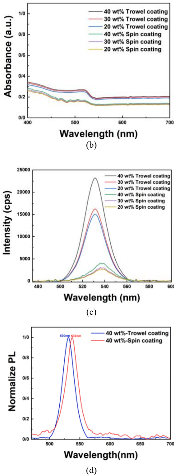
Figure 5. (a) XRD patterns of the MAPbBr_3 thin films, (b) absorption spectra, (c) Photoluminescence spectra in different concentrations and, (d) shift peak PL in 40 wt% concentration in two coating methods.
