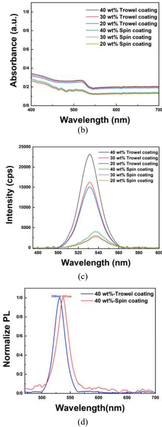
Figure 5. (a) XRD patterns of the MAPbBr_3 thin films, (b) absorption spectra, (c) Photoluminescence spectra in different concentrations and, (d) shift peak PL in 40 wt% concentration in two coating methods.
