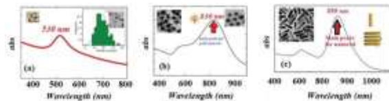
Figure 5. UV-vis Spectrum and particle shape of a) Au-NPs, b) Au-NSs, and c) Au-NRs.
