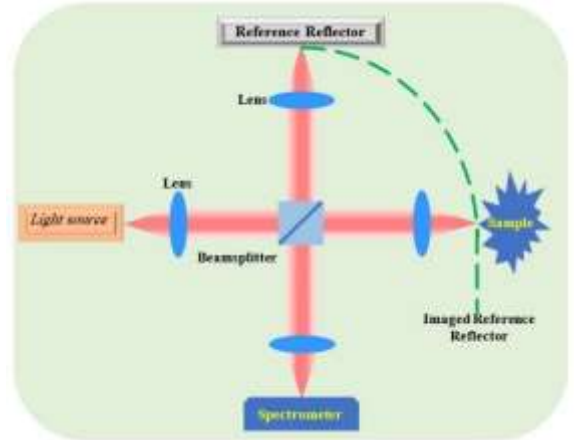
Figure 3. Michelson interferometer for FD-OCT experiment.
