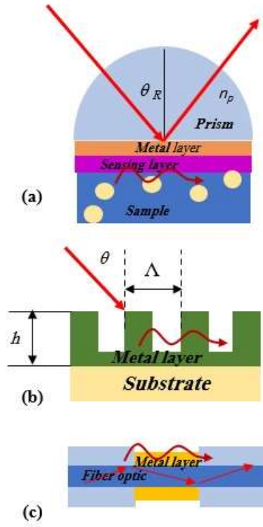
Figure 4. a) prism coupling, b) grating coupling, and c) waveguide coupling [58].
